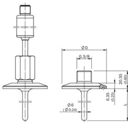
Complete assembly
