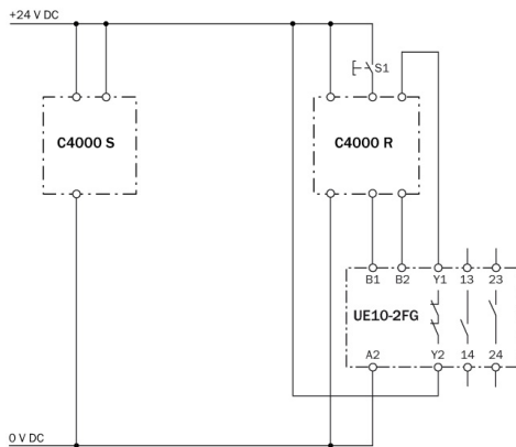
Connection diagram
