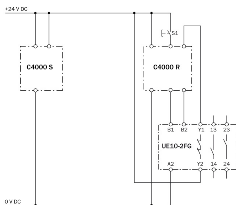
Connection diagram
