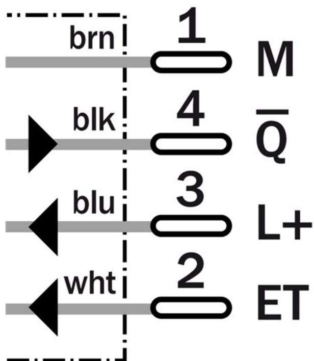
Connection diagram
