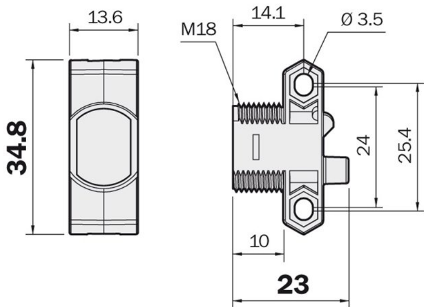
Dimensional drawing
