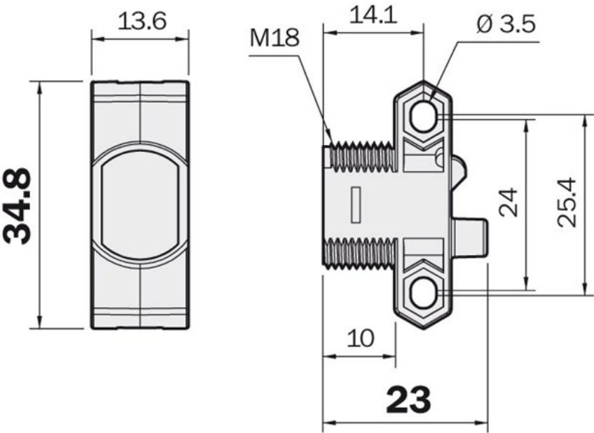
Dimensional drawing
