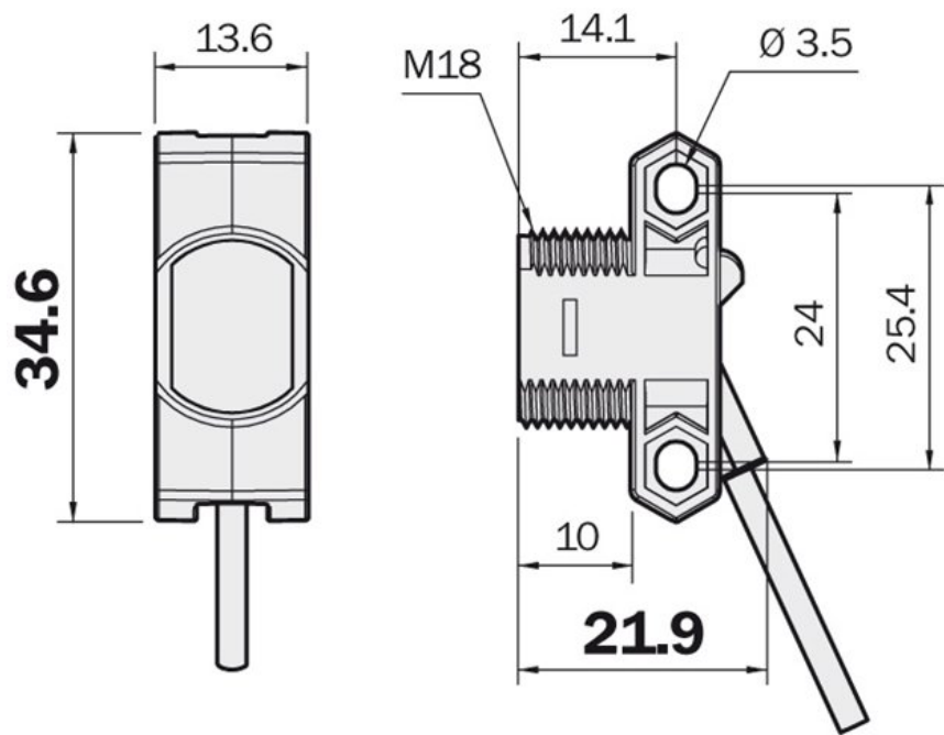
Dimensional drawing
