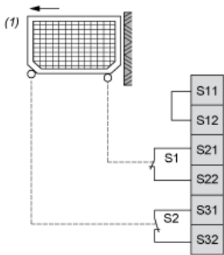
(1) Protective guard
