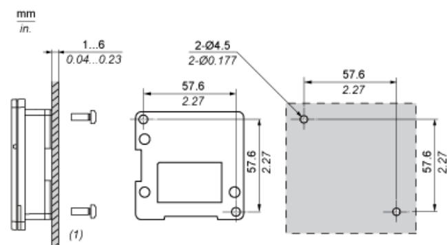
(1) Installation panel
