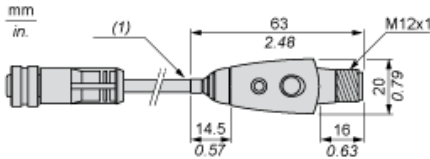
(1) Cable, length: 152 mm.
